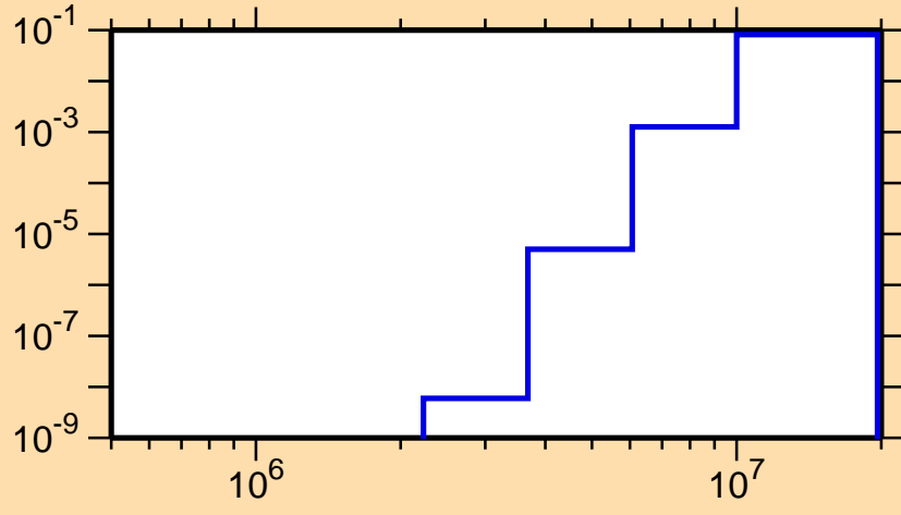
\sigma vs. E for ^{97}\text{Ag}(n,p\alpha)
