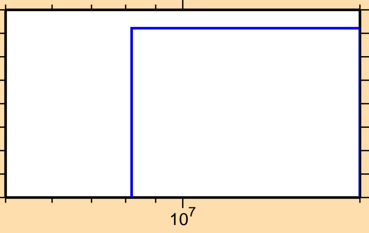
\sigma vs. E for ^{97}\text{Ag}(n,2np)
