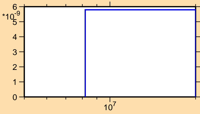
\sigma vs. E for ^{97}\text{Ag} (mt 45)
