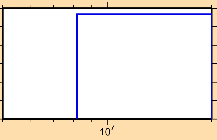
\sigma vs. E for ^{97}\text{Ag}(n,\text{nd})
