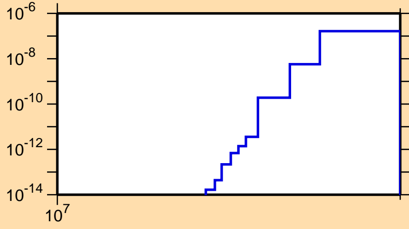
\sigma vs. E for ^{98}\text{Ag}(\text{mt } 34)
