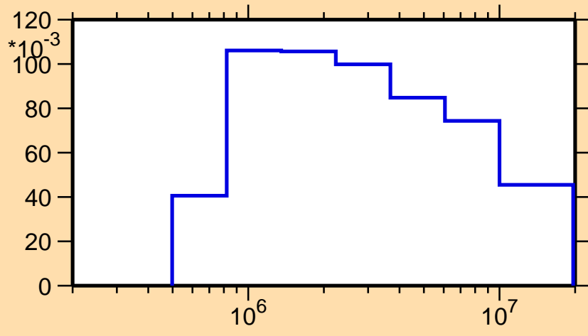
\sigma vs. E for ^{98}\text{Ag}(n,n_4)
