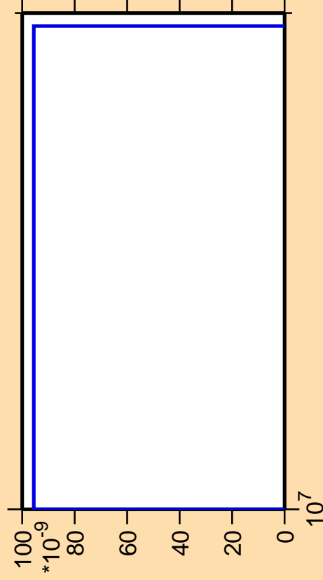
\Delta\sigma/\sigma vs. E for ^{98}\text{Ag}(n,nt)
