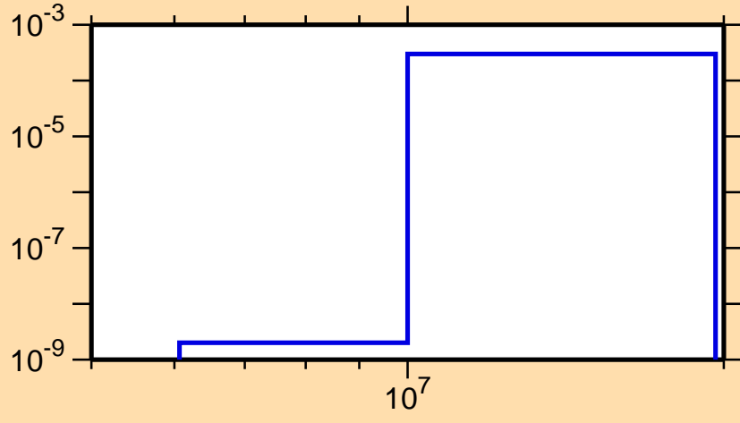
\sigma vs. E for ^{98}\text{Ag}(n,n\alpha)
