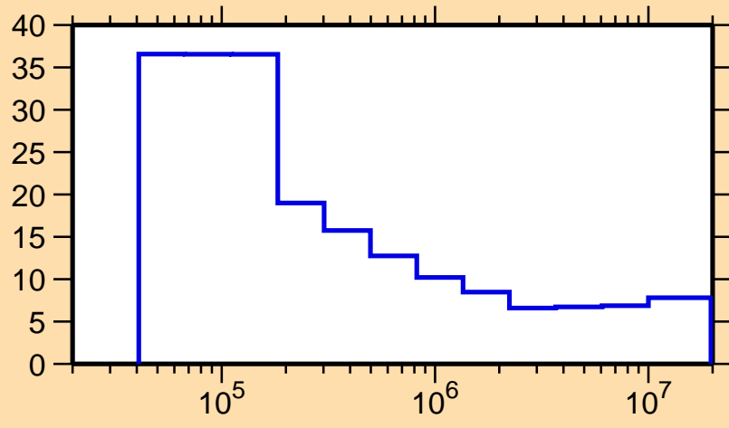
\Delta\sigma/\sigma vs. E for ^{98}\text{Ag}(n,\text{nonel.})
