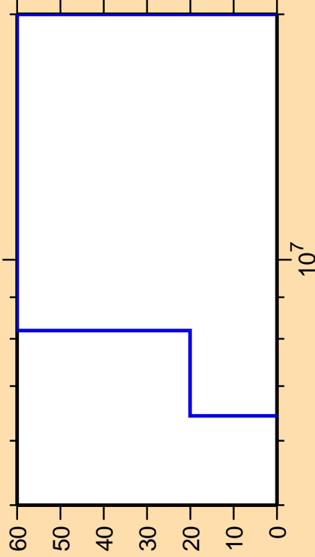
\Delta\sigma/\sigma vs. E for ^{98}\text{Ag}(n,n\alpha)
