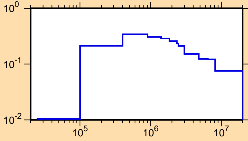
\sigma vs. E for ^{98}\text{Ag}(n,\text{inel.})
