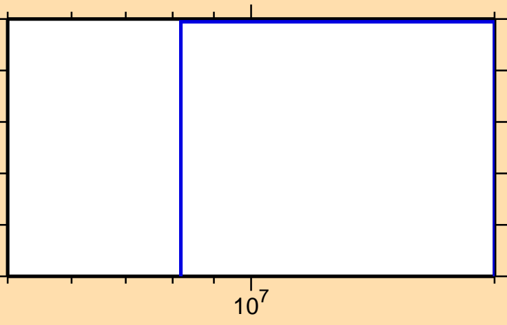
\sigma vs. E for ^{98}\text{Ag}(n,\text{pd})
