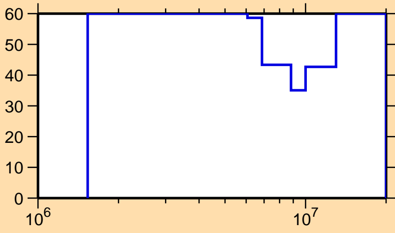
\Delta\sigma/\sigma vs. E for ^{99}\text{Ag}(n,ncont.)
