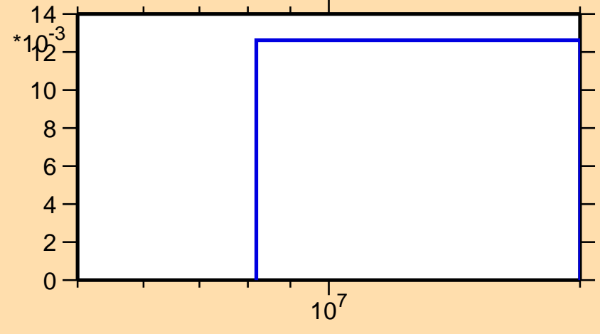
\sigma vs. E for ^{99}\text{Ag}(n,2n)
