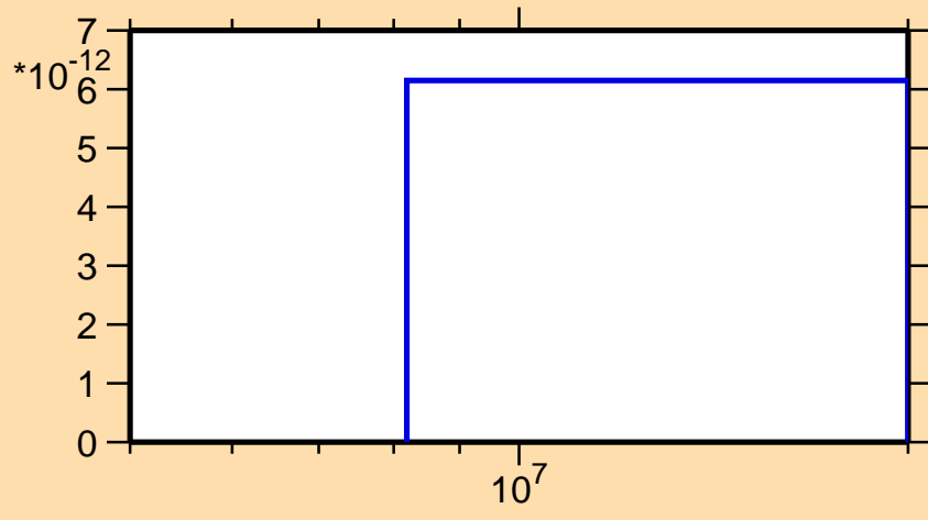
\sigma vs. E for ^{99}\text{Ag}(\text{mt } 34)
