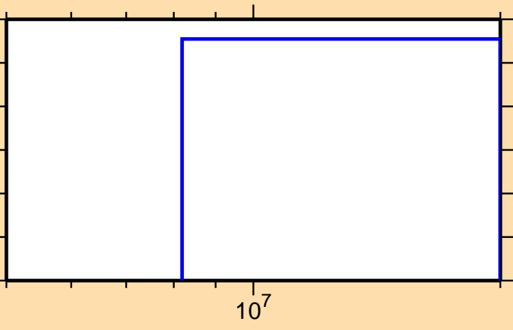
\sigma vs. E for ^{99}\text{Ag}(n,\text{pt})
