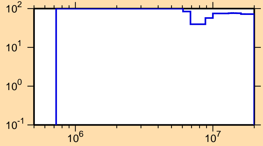
\Delta\sigma/\sigma vs. E for ^{99}\text{Ag}(n,n\text{cont.})
