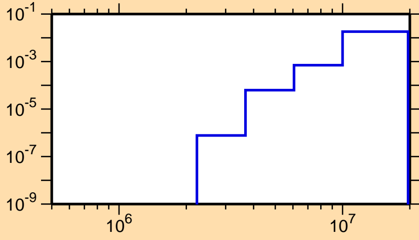
\sigma vs. E for ^{99}\text{Ag}(n,d)
