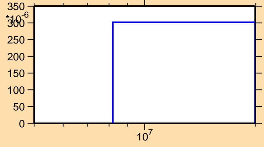
\sigma vs. E for ^{99}\text{Ag}(n,\text{pd})
