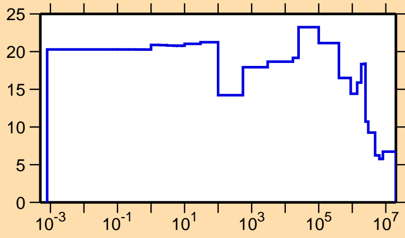
\Delta\sigma/\sigma vs. E for ^{99}\text{Ag}(n,el.)
