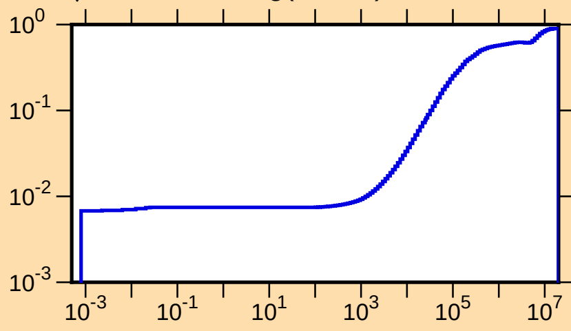
\mu vs. E for ^{100}\text{Ag}(\text{mt251})
