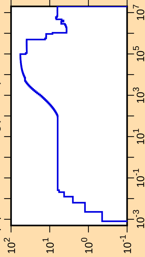
\Delta\mu/\mu vs. E for ^{100}\text{Ag}(\text{mt251})
