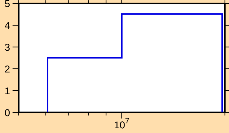
\Delta\sigma/\sigma vs. E for ^{100}\text{Ag}(n,\text{tot.})
