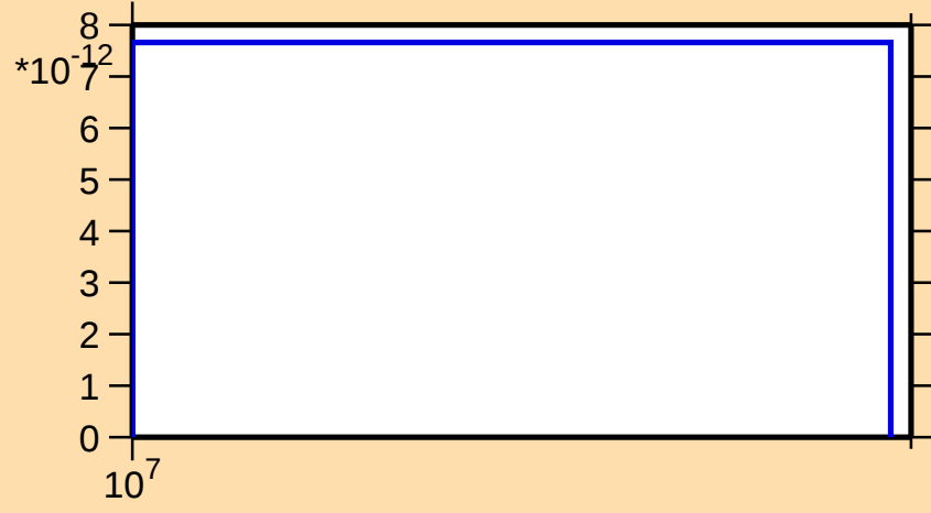
\sigma vs. E for ^{100}\text{Ag}(n,nt)
