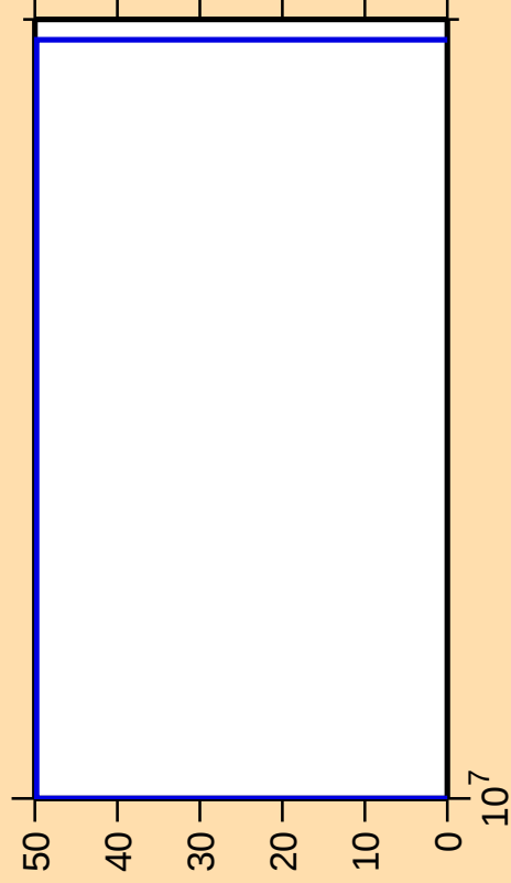
\Delta\sigma/\sigma vs. E for ^{100}\text{Ag}(n,2np)
