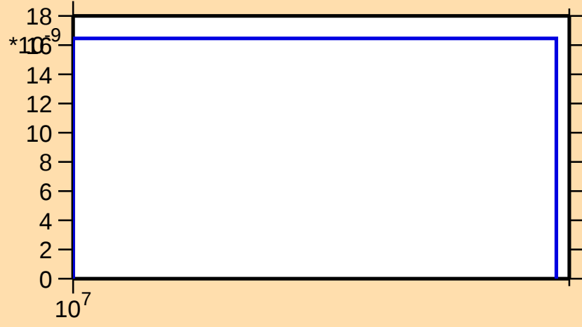
\sigma vs. E for ^{100}\text{Ag}(n,2n\alpha)
