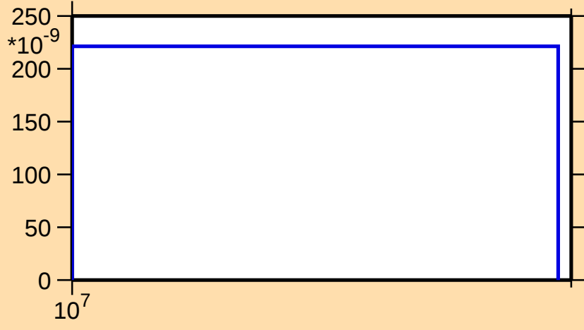
\sigma vs. E for ^{100}\text{Ag}(n,\text{pt})
