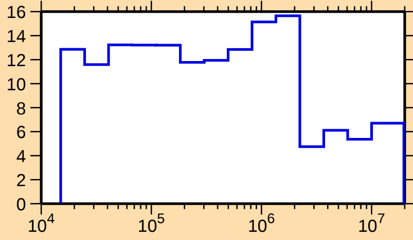
\Delta\sigma/\sigma vs. E for ^{100}\text{Ag}(n,\text{el.})
