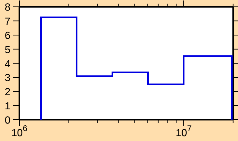
\Delta\sigma/\sigma vs. E for ^{100}\text{Ag}(n,\text{tot.})
