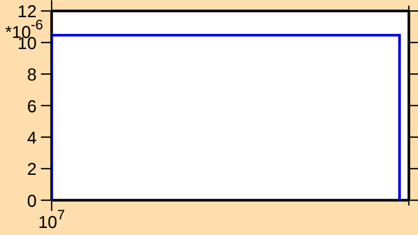
\sigma vs. E for ^{100}\text{Ag}(n,\text{nd})
