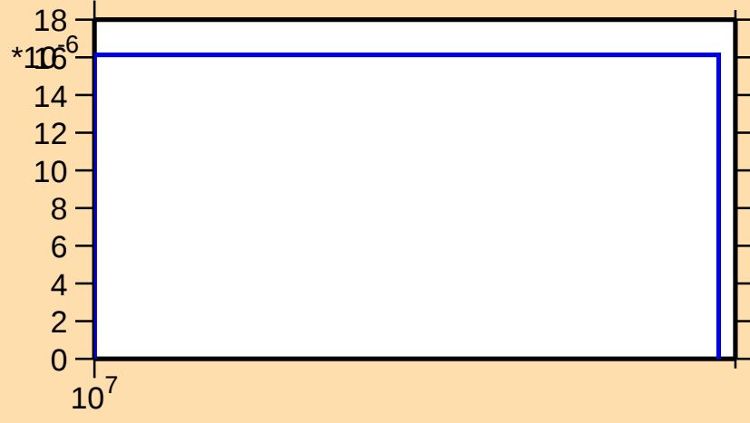
\sigma vs. E for ^{100}\text{Ag}(n,\text{pd})
