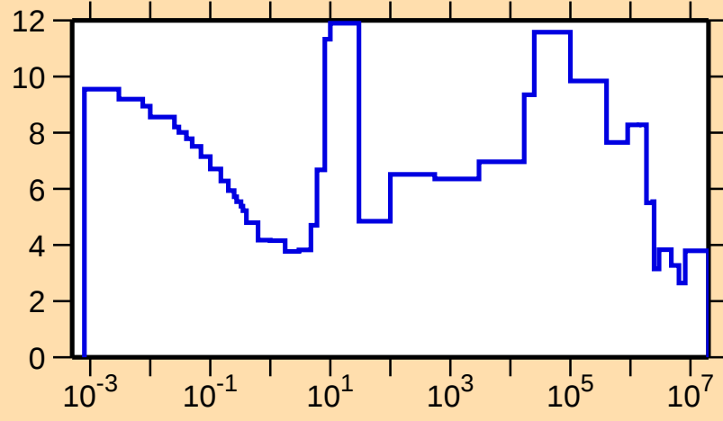
\Delta\sigma/\sigma vs. E for ^{100}\text{Ag}(n,\text{tot.})
