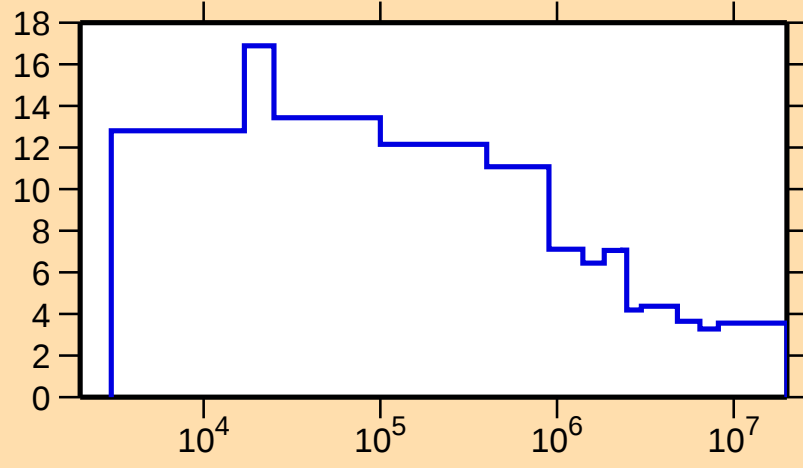
\Delta\sigma/\sigma vs. E for ^{100}\text{Ag}(n,\text{nonel.})
