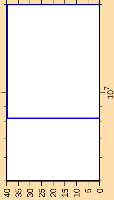
\Delta\sigma/\sigma vs. E for ^{100}\text{Ag}(n,2n)
