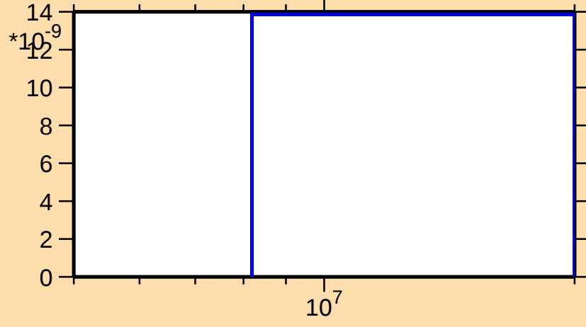
\sigma vs. E for ^{100}\text{Ag}(n,2n\alpha)
