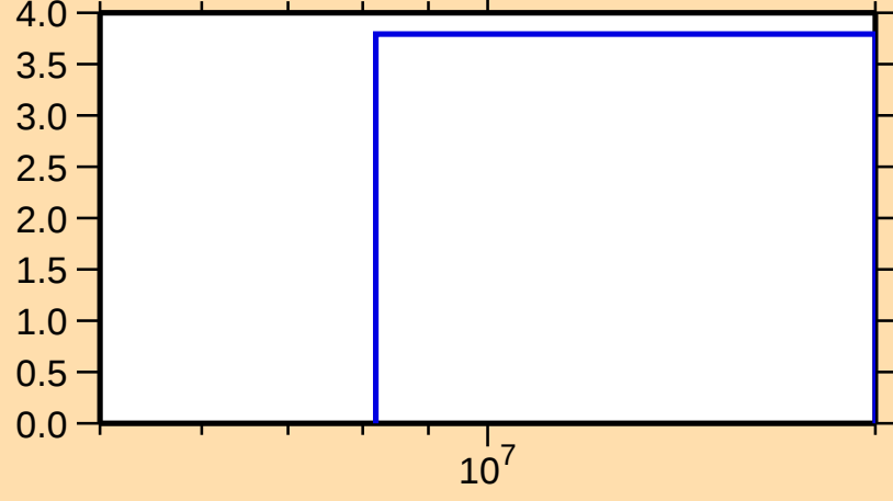
\Delta\sigma/\sigma vs. E for ^{100}\text{Ag}(n,\text{tot.})
