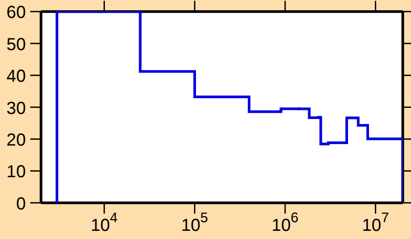
\Delta\sigma/\sigma vs. E for ^{100}\text{Ag}(n,n_1)
