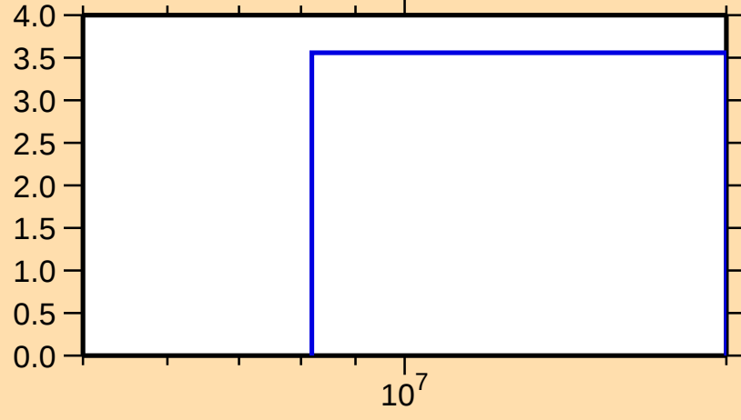
\Delta\sigma/\sigma vs. E for ^{100}\text{Ag}(n,\text{nonel.})
