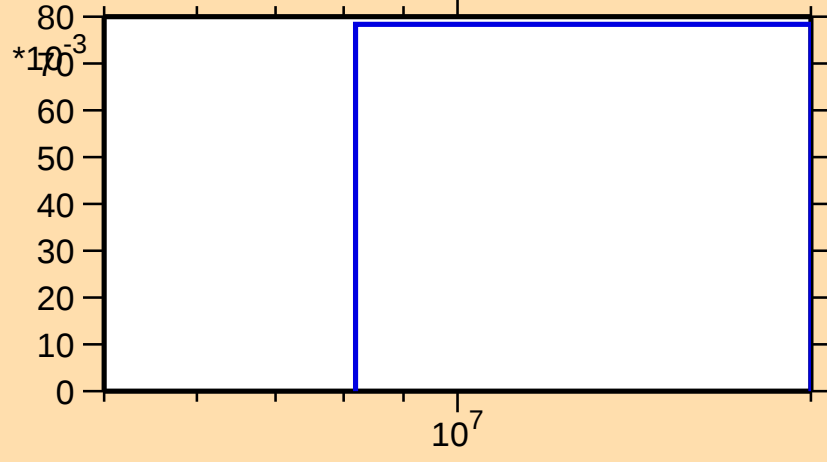
\sigma vs. E for ^{100}\text{Ag}(n,2n)
