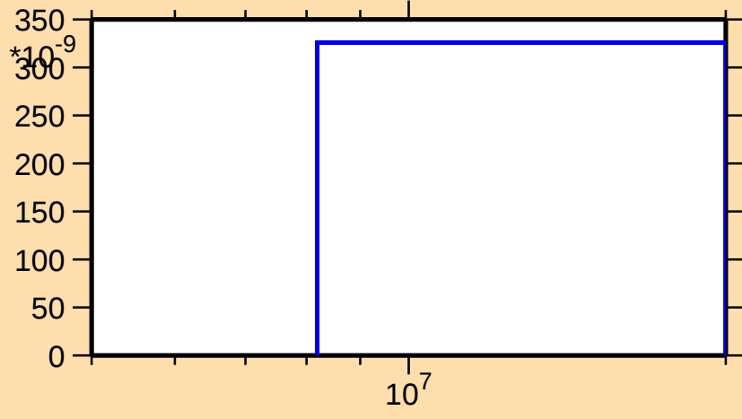
\sigma vs. E for ^{100}\text{Ag}(\text{mt117})
