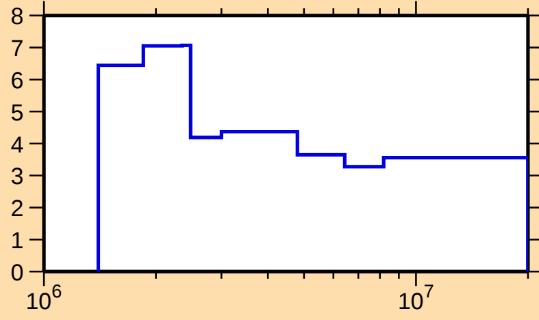
\Delta\sigma/\sigma vs. E for ^{100}\text{Ag}(n,\text{nonel.})
