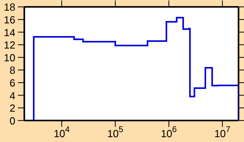
\Delta\sigma/\sigma vs. E for ^{100}\text{Ag}(n,\text{el.})
