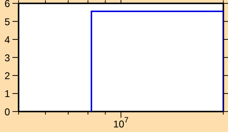
\Delta\sigma/\sigma vs. E for ^{100}\text{Ag}(n,\text{el.})
