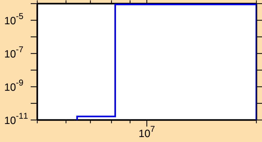
\sigma vs. E for ^{100}\text{Ag}(n,\text{He}3)
