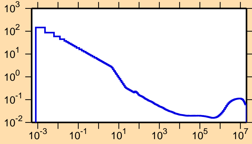
\sigma vs. E for ^{100}\text{Ag}(n,\alpha)
