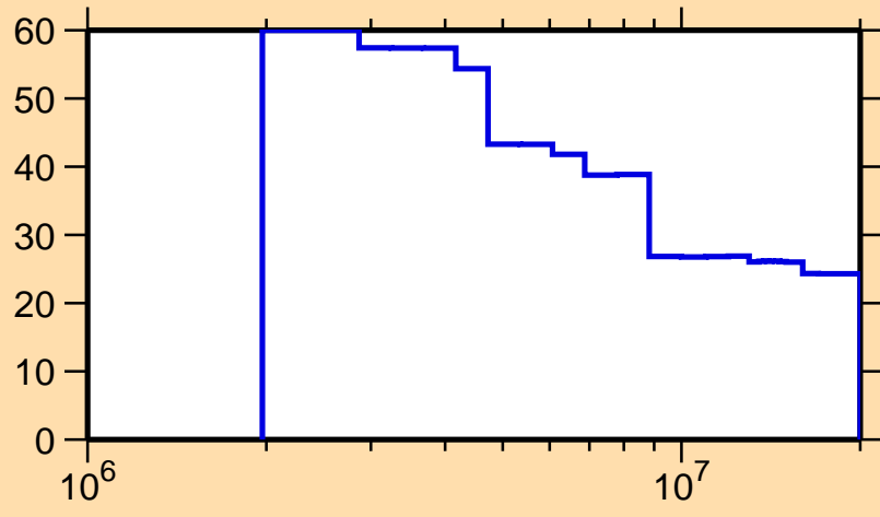
\Delta\sigma/\sigma vs. E for ^{100}\text{Ag}(n,n\text{cont.})
