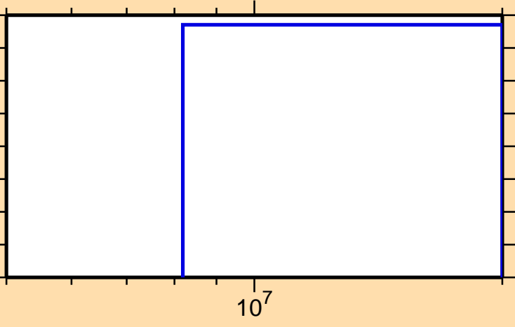
\sigma vs. E for ^{100}\text{Ag}(n,2n)
