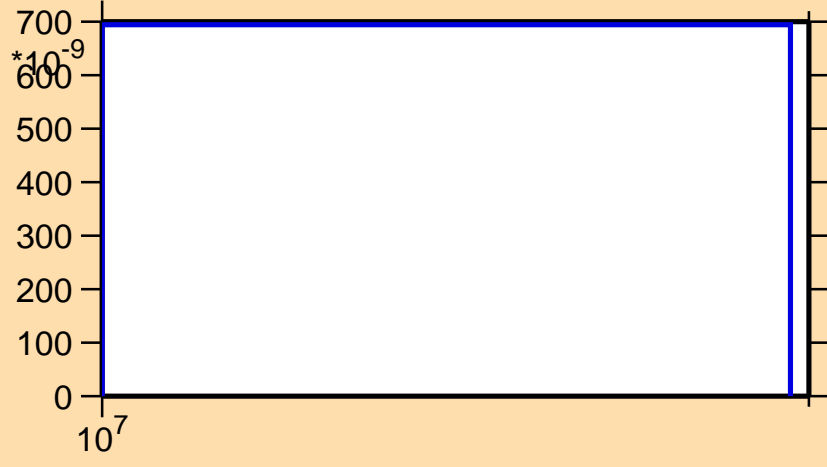
\sigma vs. E for ^{101}\text{Ag}(\text{mt } 45)
