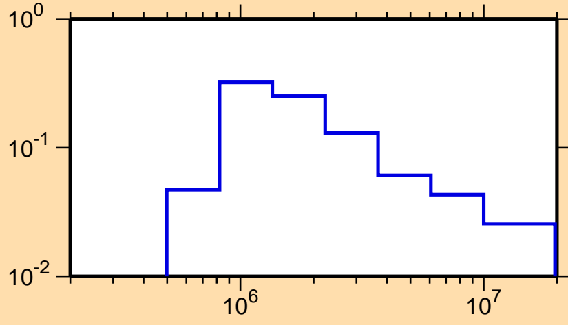
\sigma vs. E for ^{101}\text{Ag}(n,n_3)
