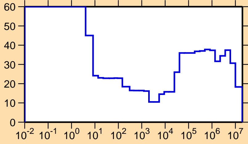
\Delta\sigma/\sigma vs. E for ^{101}\text{Ag}(n,p)
