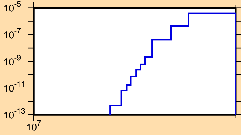
\sigma vs. E for ^{102}\text{Ag}(n,pd)
