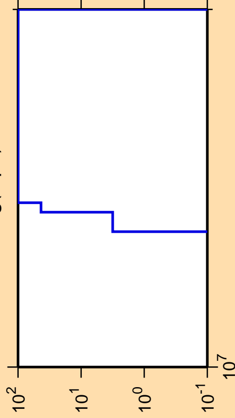
\Delta\sigma/\sigma vs. E for ^{102}\text{Ag}(n,pd)
