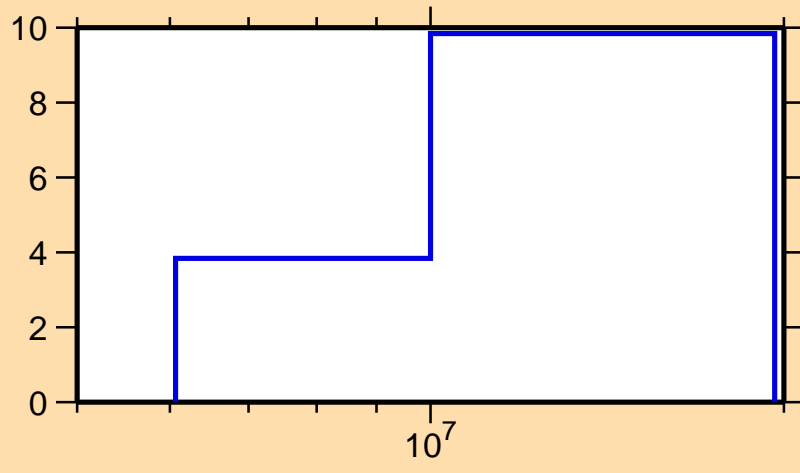
\Delta\sigma/\sigma vs. E for ^{102}\text{Ag}(n,\text{tot.})
