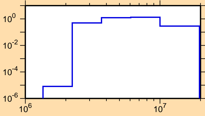
\sigma vs. E for ^{102}\text{Ag}(n,n\text{cont.})
