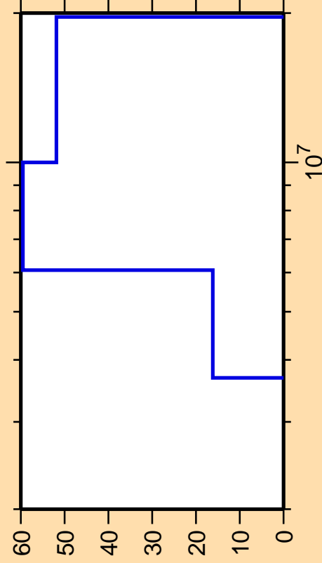
\Delta\sigma/\sigma vs. E for ^{102}\text{Ag}(n,n\alpha)
