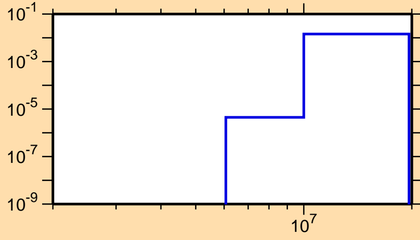
\sigma vs. E for ^{102}\text{Ag}(n,n\alpha)
