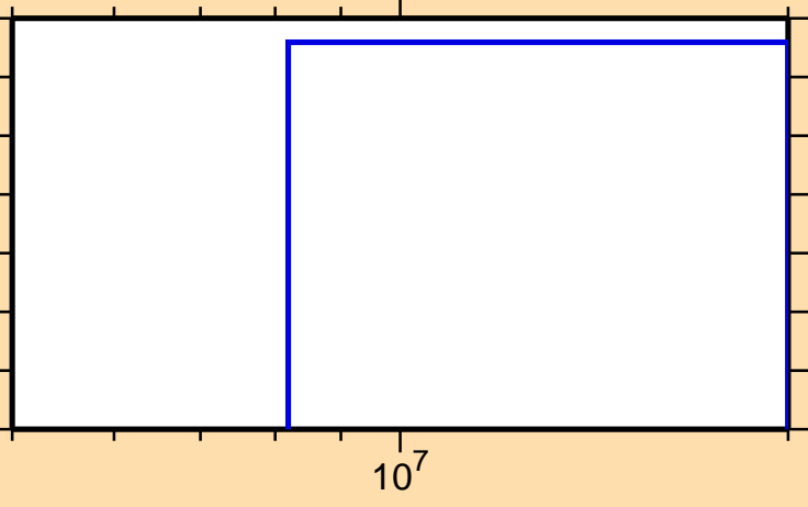
\sigma vs. E for ^{102}\text{Ag}(n,\text{nd})
