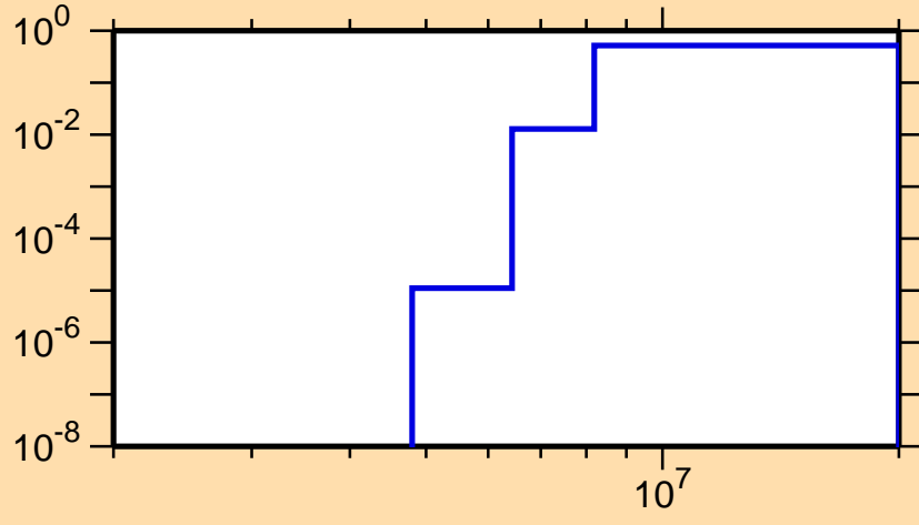
\sigma vs. E for ^{103}\text{Ag}(n,np)
