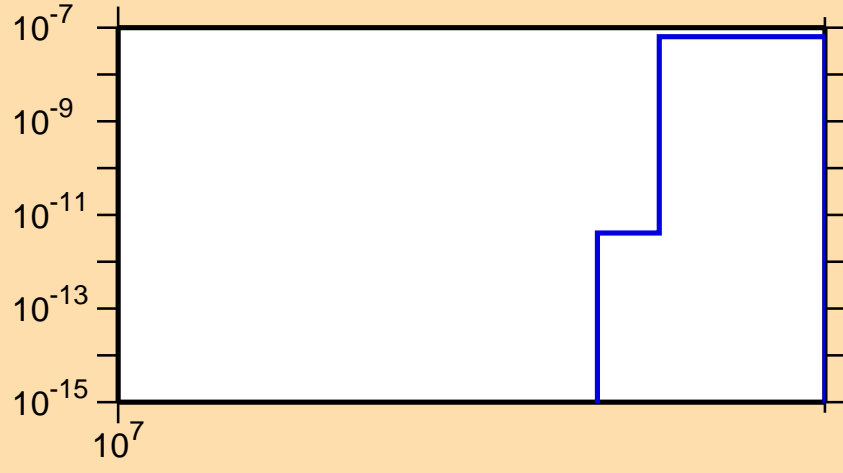
\sigma vs. E for ^{103}\text{Ag}(n,nt)
