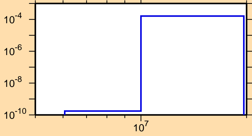
\sigma vs. E for ^{103}\text{Ag}(n,t)
