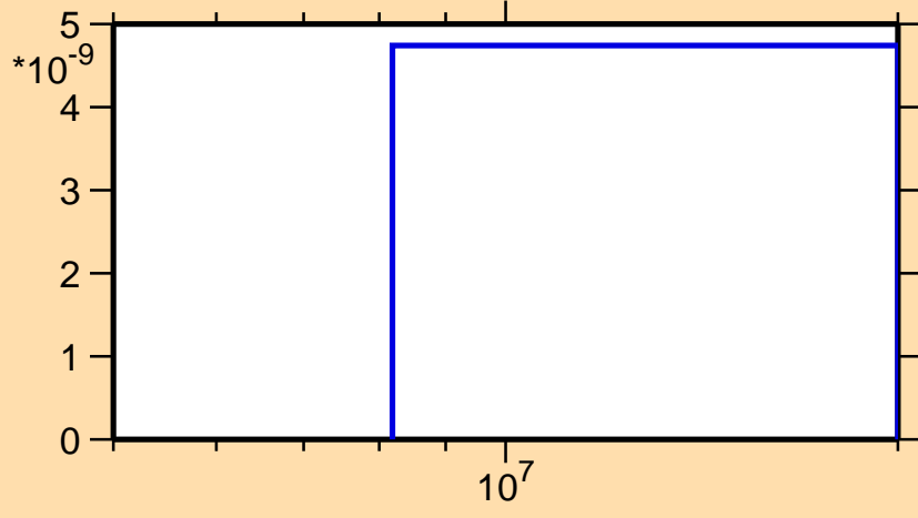
\sigma vs. E for ^{103}\text{Ag}(\text{mt117})
