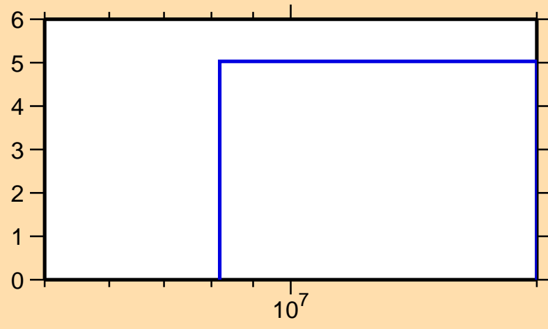
\Delta\sigma/\sigma vs. E for ^{103}\text{Ag}(n,\text{tot.})
