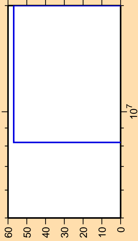
\Delta\sigma/\sigma vs. E for ^{103}\text{Ag}(n,pd)
