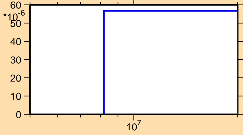
\sigma vs. E for ^{103}\text{Ag}(n,2np)
