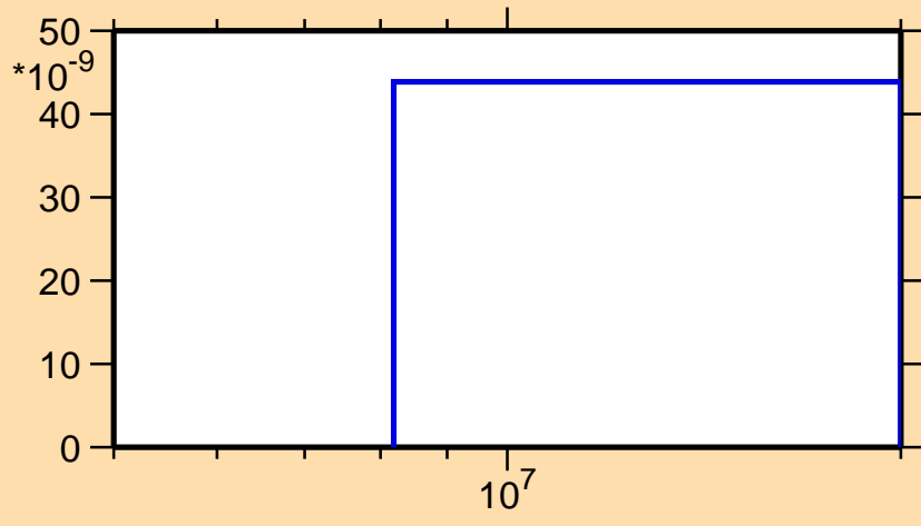
\sigma vs. E for ^{103}\text{Ag}(n,3n)
