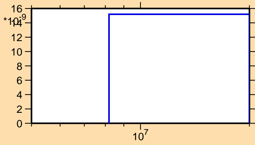
\sigma vs. E for ^{103}\text{Ag}(n,pd)
