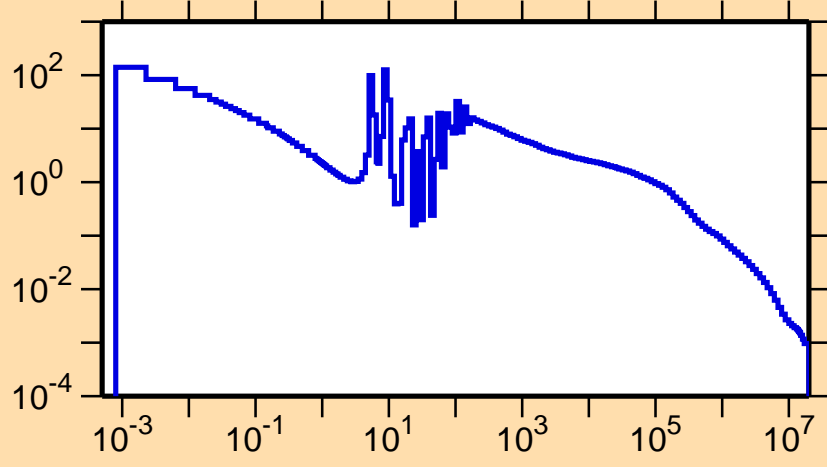
\sigma vs. E for ^{104}\text{Ag}(n,\gamma)
