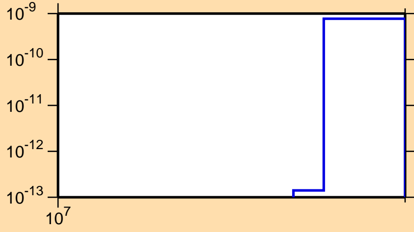
\sigma vs. E for ^{104}\text{Ag}(n,\text{pt})
