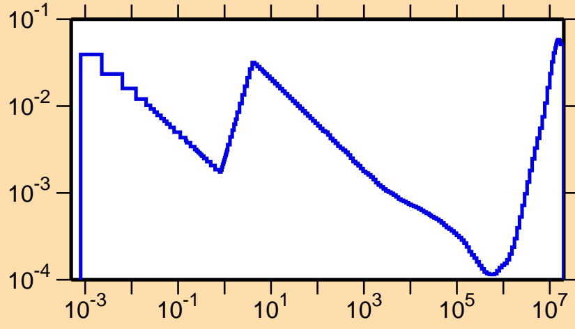
\sigma vs. E for ^{104}\text{Ag}(n,\alpha)
