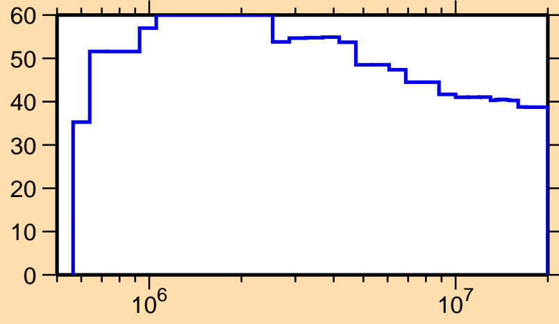
\Delta\sigma/\sigma vs. E for ^{104}\text{Ag}(n,n_1)
