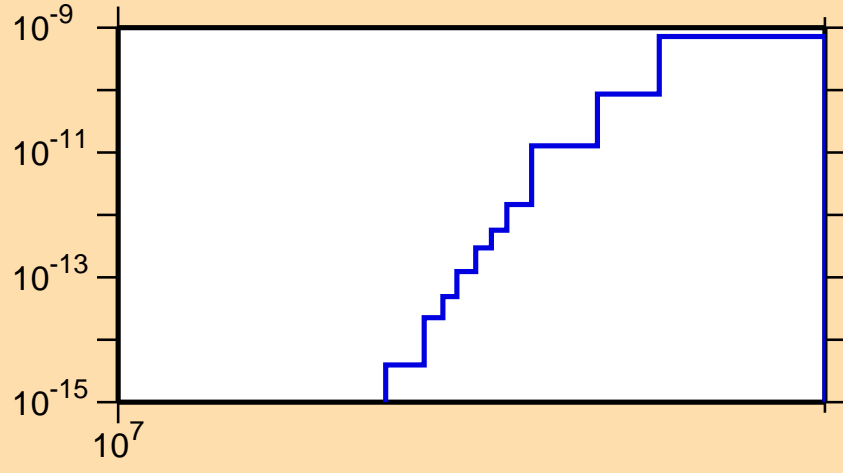
\sigma vs. E for ^{104}\text{Ag}(\text{mt117})
