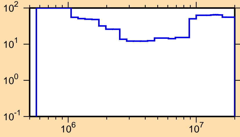
\Delta\sigma/\sigma vs. E for ^{104}\text{Ag}(n,n\text{cont.})
