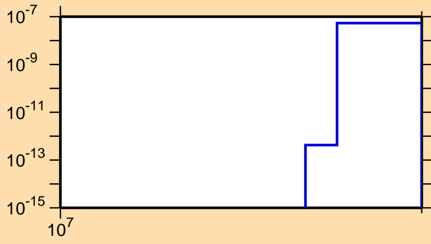
\sigma vs. E for ^{104}\text{Ag}(n,nt)
