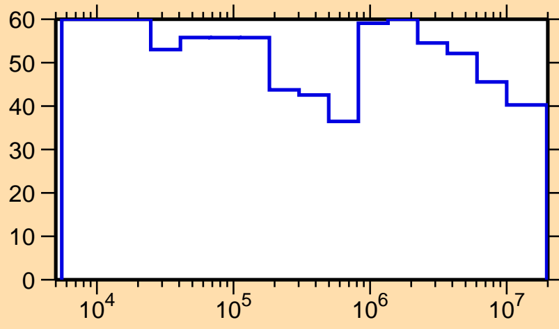
\Delta\sigma/\sigma vs. E for ^{104}\text{Ag}(n,n_1)
