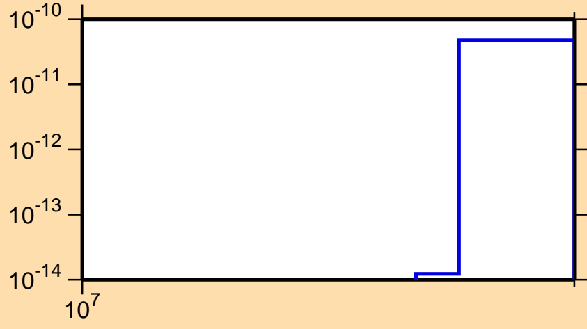
\sigma vs. E for ^{104}\text{Ag}(\text{mt } 34)
