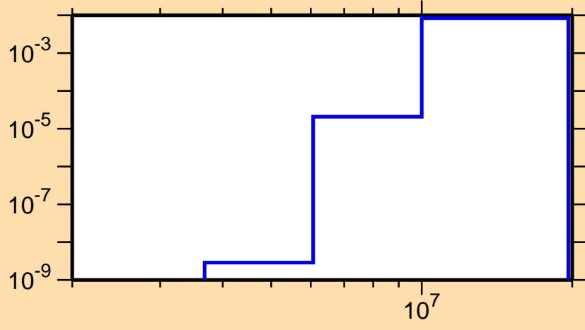
\sigma vs. E for ^{104}\text{Ag}(n,d)
