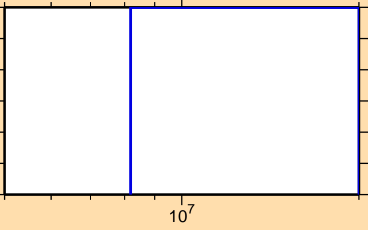
\sigma vs. E for ^{104}\text{Ag}(n,2np)
