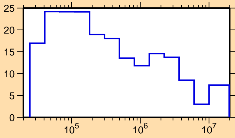
\Delta\sigma/\sigma vs. E for ^{105}\text{Ag}(n,\text{tot.})
