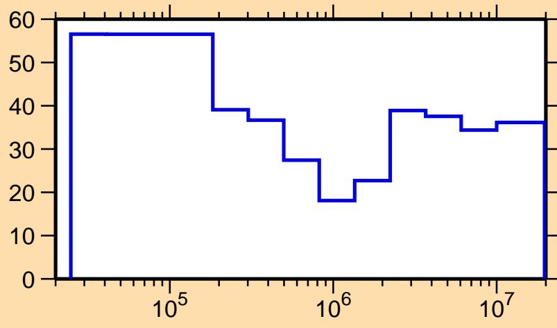
\Delta\sigma/\sigma vs. E for ^{105}\text{Ag}(n,n_1)
