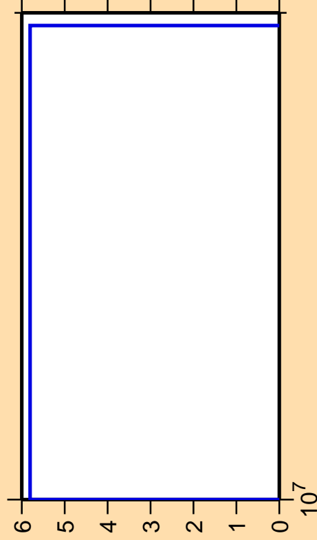
\Delta\sigma/\sigma vs. E for ^{105}\text{Ag}(n,\text{pd})
