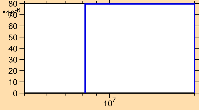
\sigma vs. E for ^{105}\text{Ag}(n,t)
