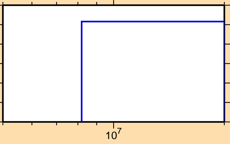
\sigma vs. E for ^{105}\text{Ag}(n,3n)
