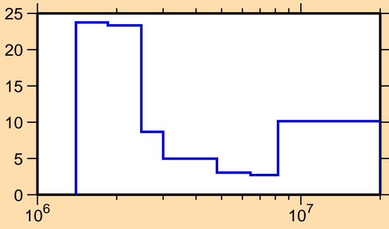
\Delta\sigma/\sigma vs. E for ^{105}\text{Ag}(n,n\text{cont.})
