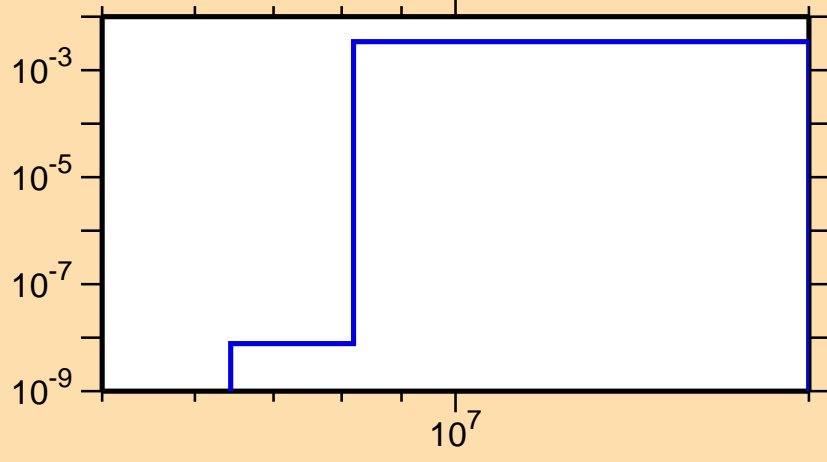
\sigma vs. E for ^{105}\text{Ag}(n,n\alpha)
