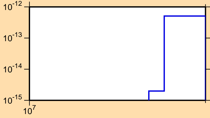
\sigma vs. E for ^{106}\text{Ag} (mt 34)
