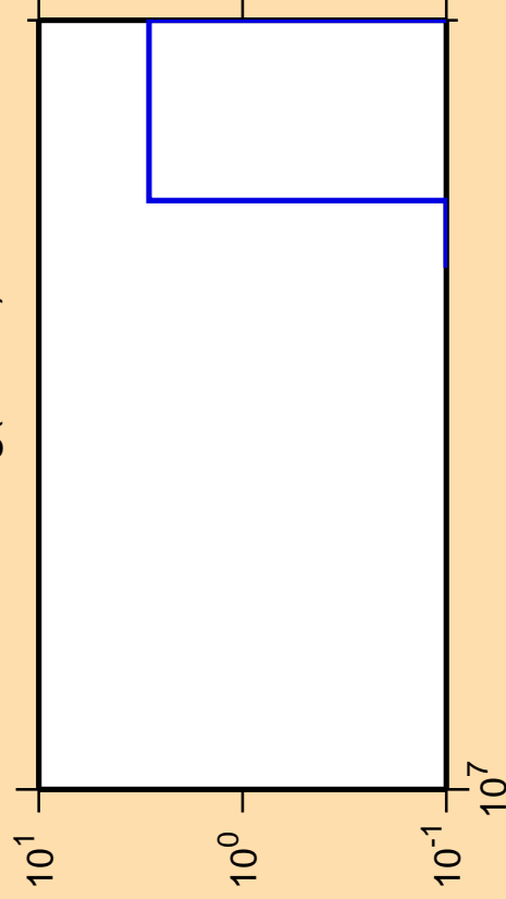
\Delta\sigma/\sigma vs. E for ^{106}\text{Ag} (mt 34)
