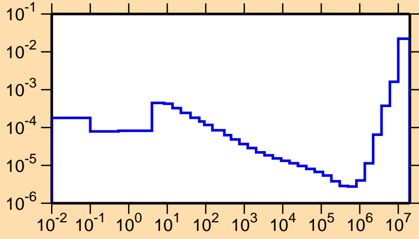
\sigma vs. E for ^{106}\text{Ag}(n,\alpha)
