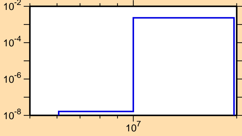
\sigma vs. E for ^{106}\text{Ag}(n,n\alpha)
