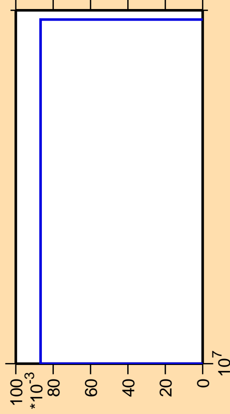
\Delta\sigma/\sigma vs. E for ^{106}\text{Ag}(n,pd)
