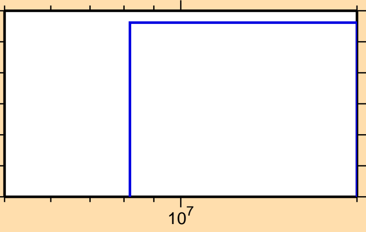
\sigma vs. E for ^{106}\text{Ag}(n,\text{He}3)
