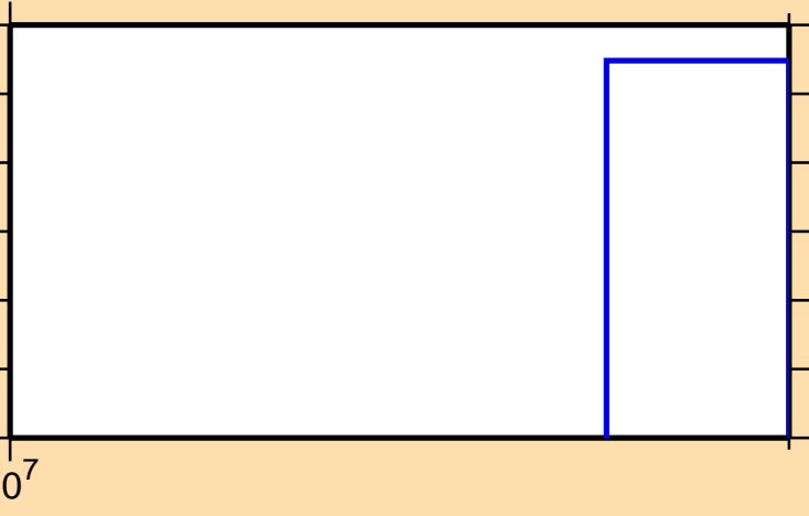
\sigma vs. E for ^{106}\text{Ag}(n,3n)
