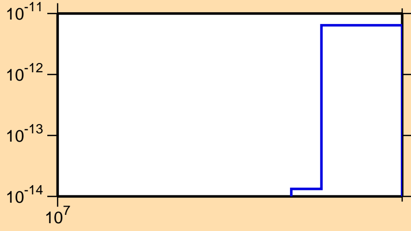
\sigma vs. E for ^{107}\text{Ag}(\text{mt } 45)
