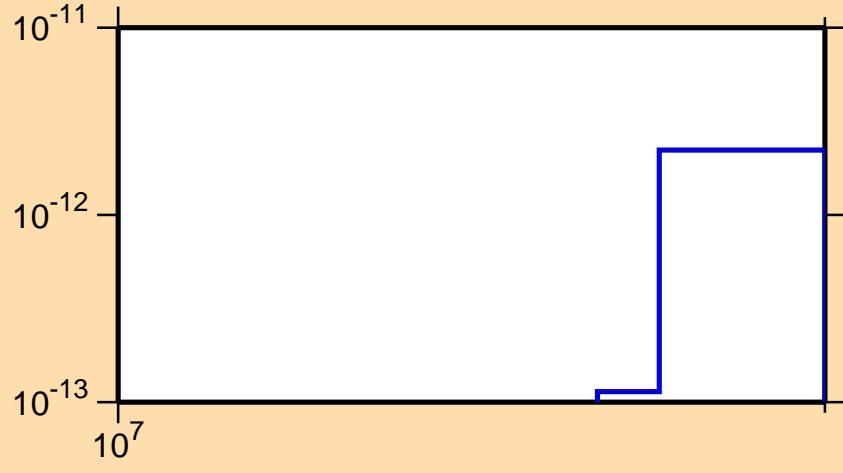
\sigma vs. E for ^{107}\text{Ag}(\text{mt117})
