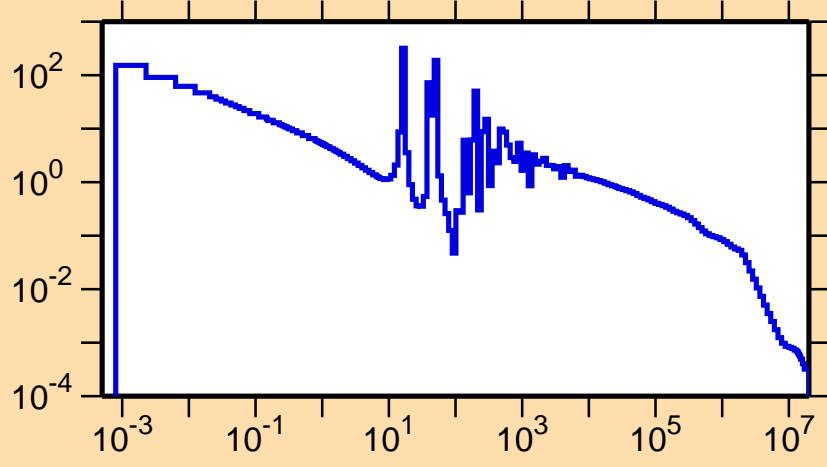
\sigma vs. E for ^{107}\text{Ag}(n,\gamma)
