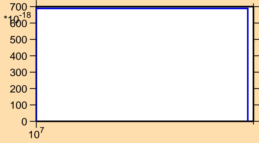
\sigma vs. E for ^{107}\text{Ag}(n,pd)
