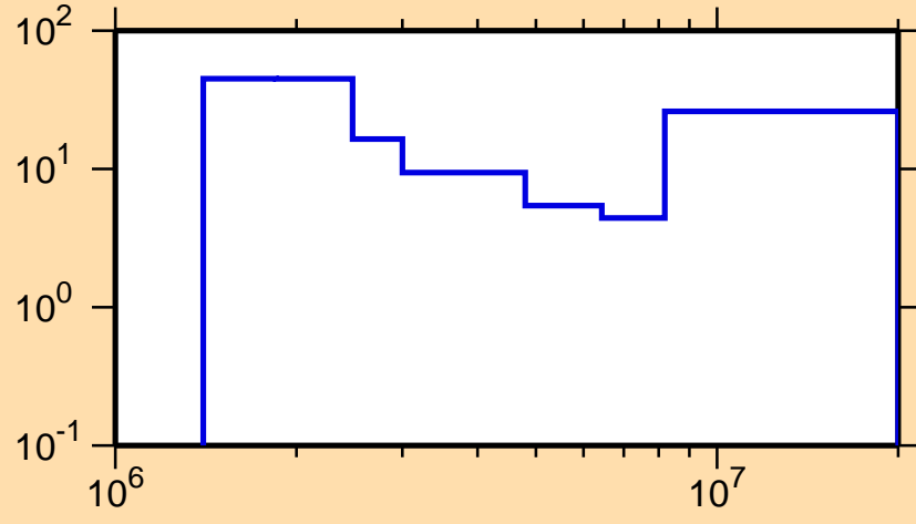
\Delta\sigma/\sigma vs. E for ^{107}\text{Ag}(n,n\text{cont.})
