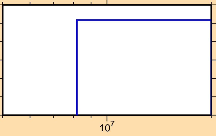
\sigma vs. E for ^{107}\text{Ag}(n,\text{nd})
