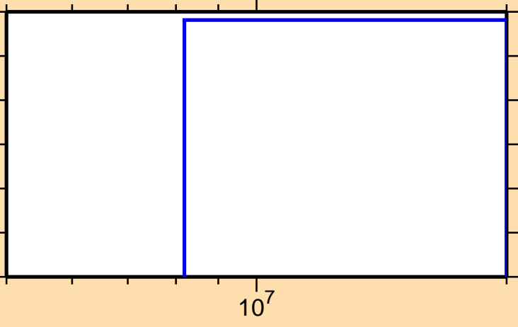
\sigma vs. E for ^{107}\text{Ag}(n,t)
