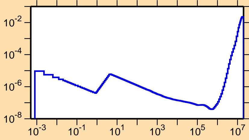
\sigma vs. E for ^{108}\text{Ag}(n,\alpha)
