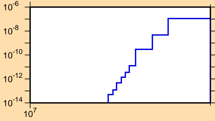
\sigma vs. E for ^{108}\text{Ag}(n,\text{He3})
