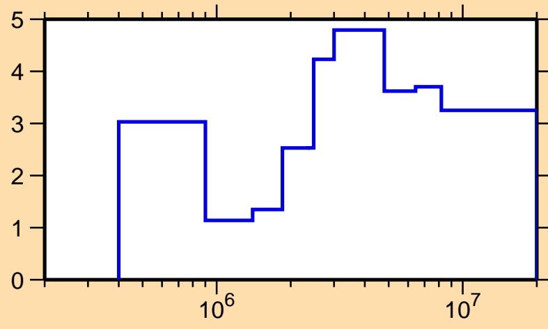
\Delta\sigma/\sigma vs. E for ^{108}\text{Ag}(n, n_{\text{nonel}})
