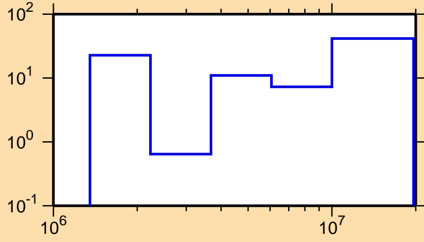
\Delta\sigma/\sigma vs. E for ^{109}\text{Ag}(n,n\text{cont.})
