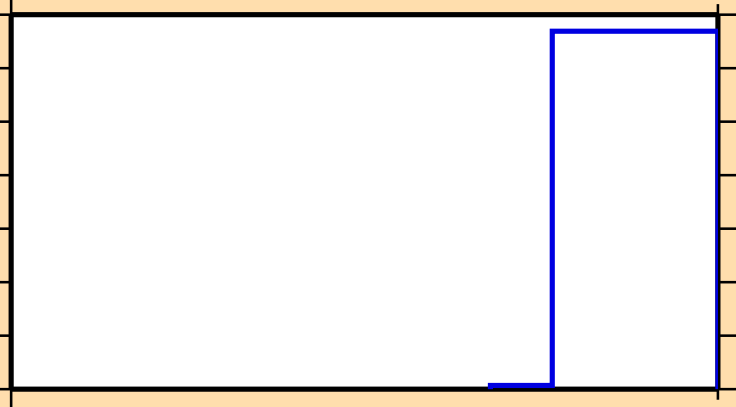
\sigma vs. E for ^{111}\text{Ag}(n,2np)
