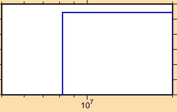
\sigma vs. E for ^{111}\text{Ag}(n,\text{nd})
