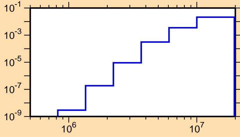
\sigma vs. E for ^{112}\text{Ag}(n,p)
