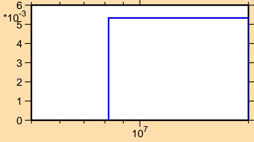
\sigma vs. E for ^{112}\text{Ag}(n,3n)
