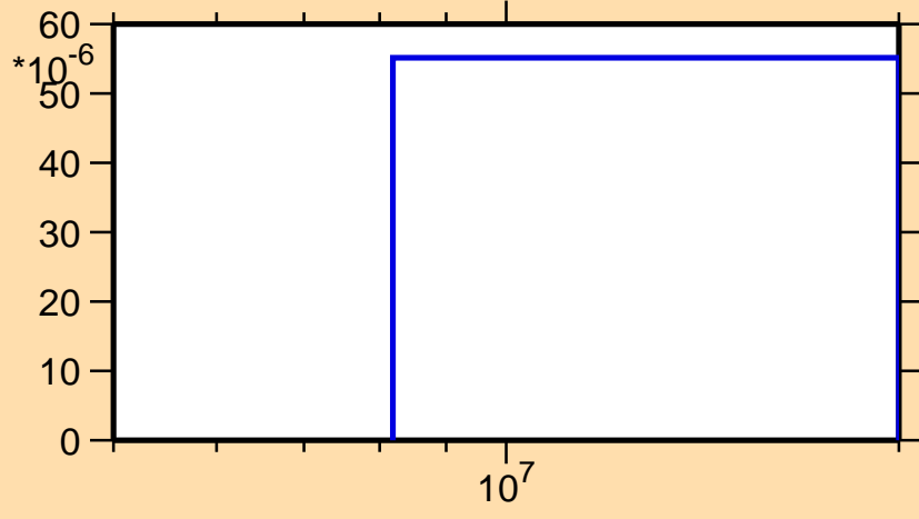
\sigma vs. E for ^{112}\text{Ag}(n,n\alpha)
