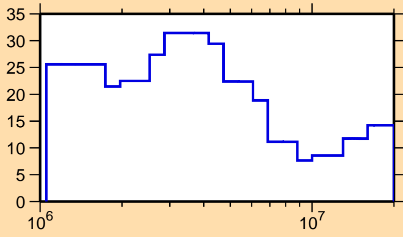
\Delta\sigma/\sigma vs. E for ^{114}\text{Ag}(n, tot.)
