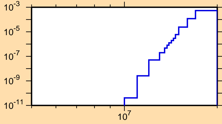
\sigma vs. E for ^{114}\text{Ag}(n,n\alpha)
