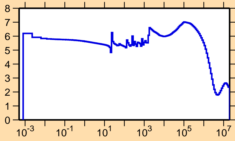
\sigma vs. E for ^{115}\text{Ag}(n,\text{el.})
