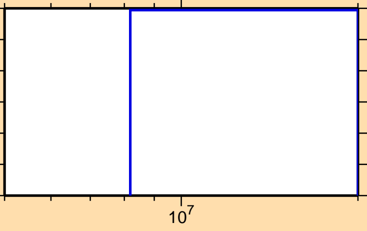
\sigma vs. E for ^{115}\text{Ag}(n,3n)
