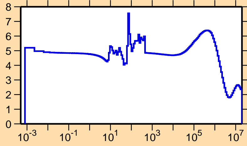
\sigma vs. E for ^{116}\text{Ag}(n,\text{el.})
