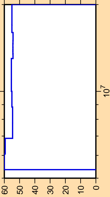
\Delta\sigma/\sigma vs. E for ^{116}\text{Ag}(n,2n)
