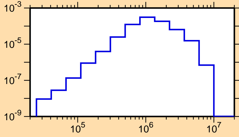
\sigma vs. E for ^{116}\text{Ag}(n,n_1)
